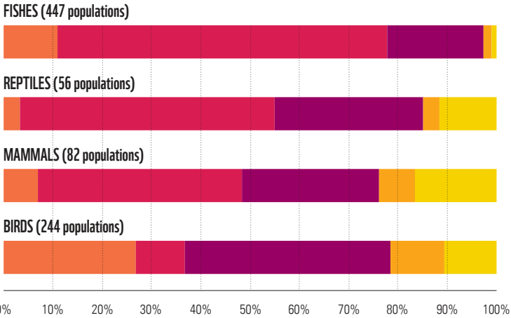
Figure 20: Taxonomic differences in threat frequency for 829 declining marine populations in the LPI database (WWF/ZSL, 2016).
