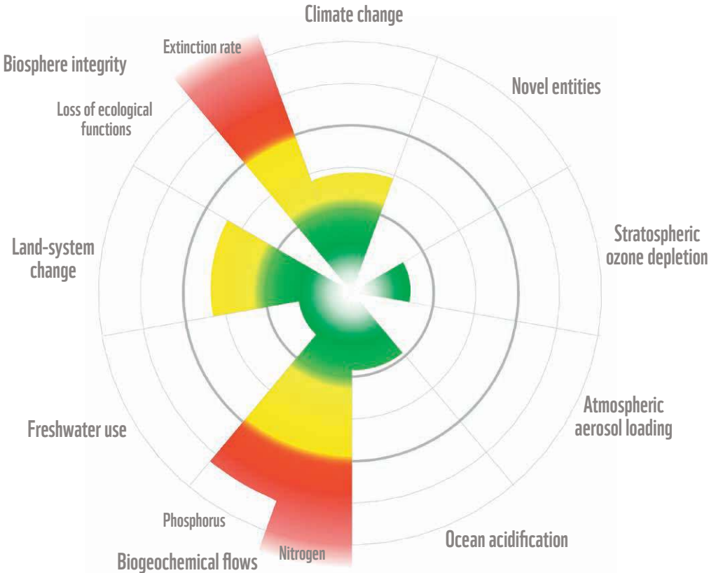
Figure 30: Planetary Boundaries
