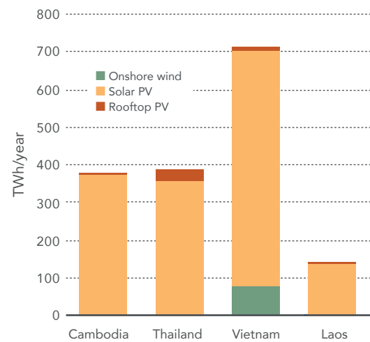
7.7. Low-impact, utility-scale wind and solar energy potential available on converted lands in countries in the Lower Mekong Basin. Modeled technologies include utility-scale wind and PV and rooftop PV.
