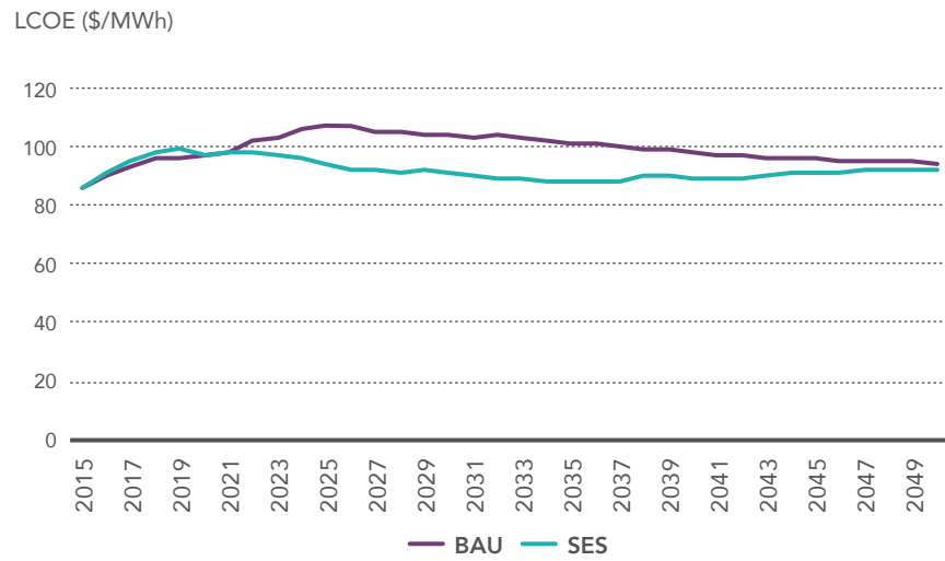
7.4. Comparing the levelized cost of electricity (LCOE) of the business-as-usual (BAU) and sustainable energy scenario (SES; from WWF 2016).
